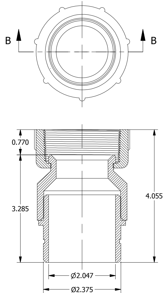
SECTION B-B
