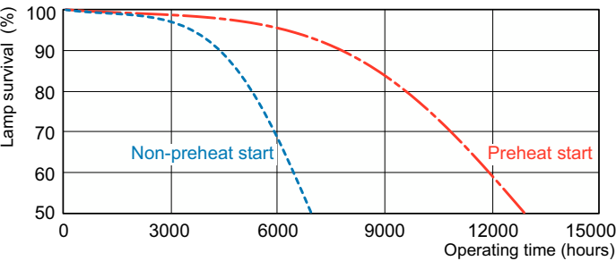
Life Expectancy Diagram - PL-T 26W/835/A/4P 1CT/5X10BOX ALTO
