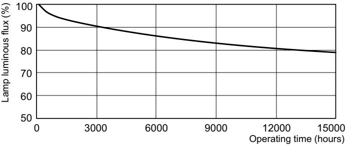
Lumen Maintenance Diagram - PL-T 32W/841/A/4P 1CT/5X10BOX ALTO
