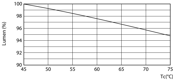
LEDtube 1200mm T8 9,5W LumenVsTc
