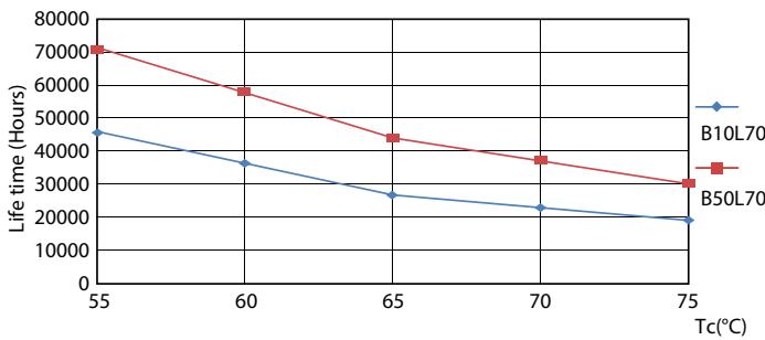
LEDtube 1200mm T8 9,5W LifetimeVsTc
