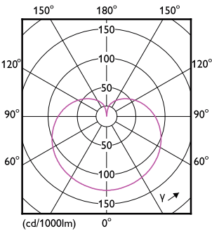
Light Distribution Diagram - 8.8A19/PER/940/P/E26/DIM 6/1FB T20
