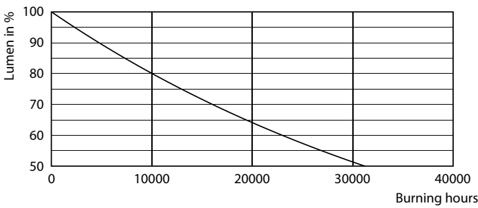
Lumen Maintenance Diagram - 8.8A19/PER/940/P/E26/DIM 6/1FB T20
