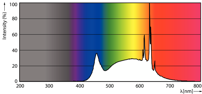
Spectral Power Distribution Colour - 8.8A19/PER/940/P/E26/DIM 6/1FB T20
