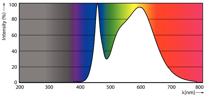
Spectral Power Distribution Colour - 14GC/LED/840/ND E26 BB 6/1
