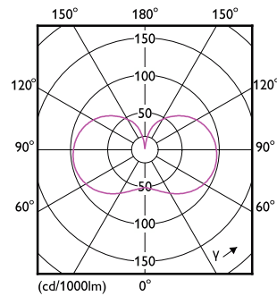
Light Distribution Diagram - 14GC/LED/840/ND E26 BB 6/1
