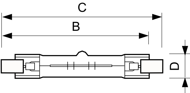
DEComp 100W R7s 120V T11 CL
