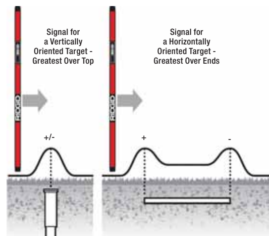
Signals and Polarity from Vertical and Horizontal Targets.
