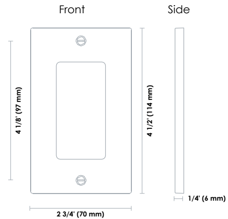
Trim Plate
