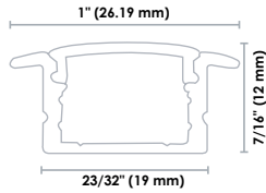
Series 210 with lens
