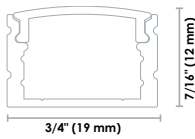
Series 200 with lens
