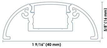
Series 300 with lens
