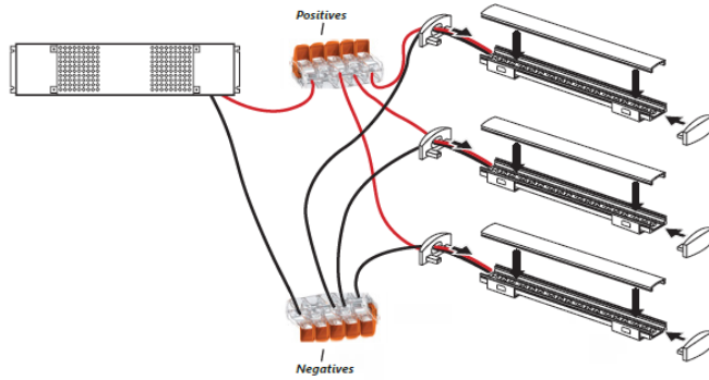
66771 - TWO WAY WAGOS
