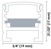
Series 400 with lens
