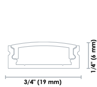
Series 100 with lens
