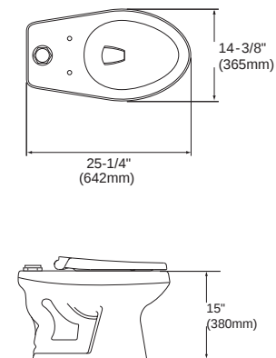
12" rough-in dimensions
