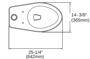
12" rough-in dimensions
