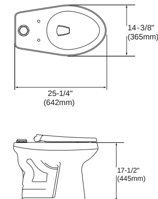
12" rough-in dimensions
