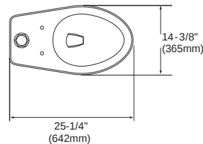
12" rough-in dimensions
