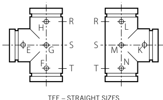
TEE – STRAIGHT SIZES
