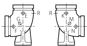
90° BASE ELBOW – STRAIGHT &amp; REDUCING
