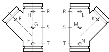
45° LATERAL – STRAIGHT &amp; REDUCING
