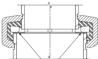
Assembly Washer
