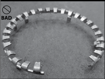
EXAMPLE OF RETAINER IN BAD CONDITION THAT SHALL NOT BE REUSED (TEETH ARE BENT, SHAPE IS DEFORMED)
