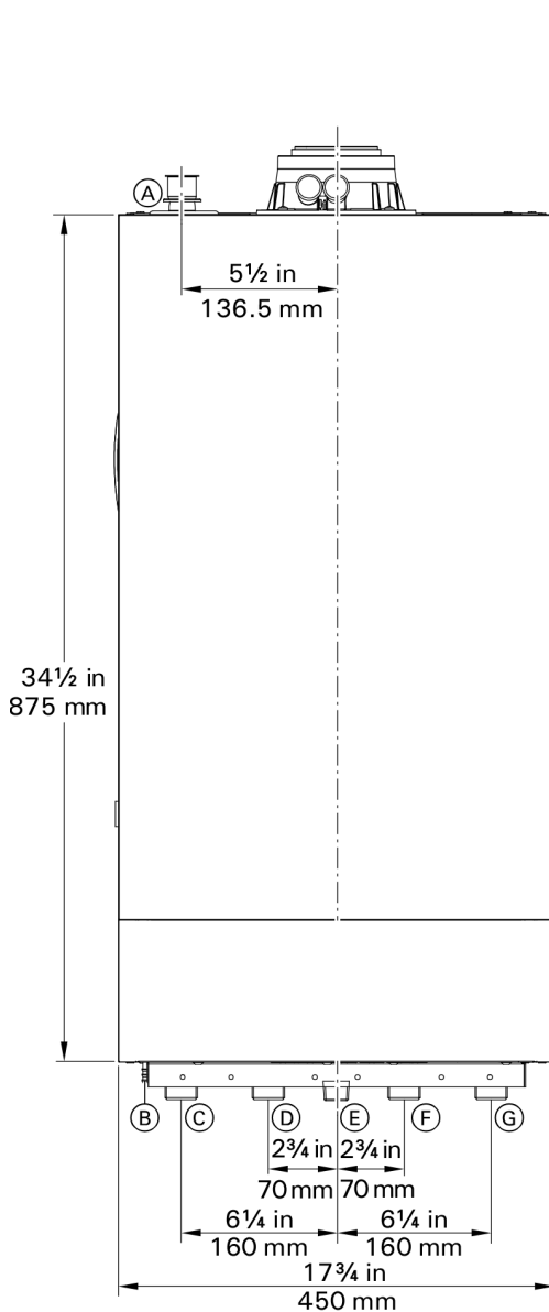
Front view
