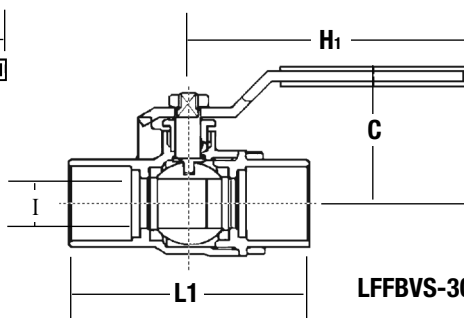
LFFBV-3C-SS
