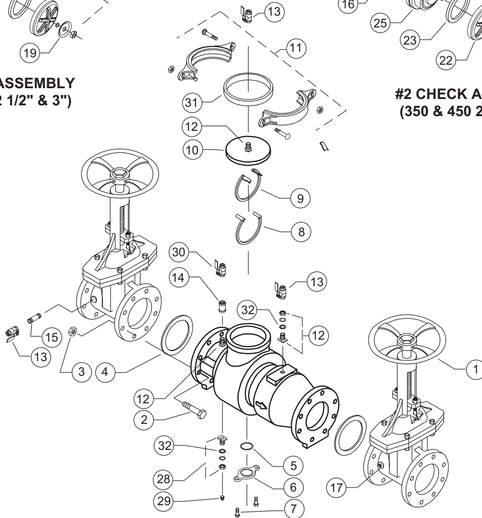
MODEL 350 (2 1/2" - 3")
