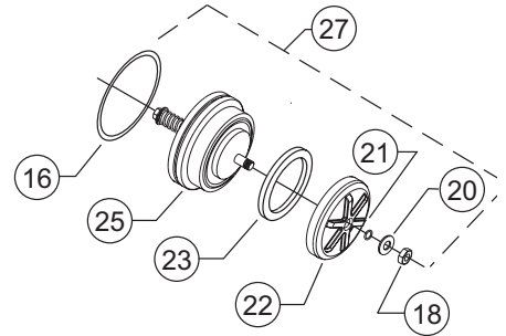
#2 CHECK ASSEMBLY (350 & 450 2 1/2" & 3")
