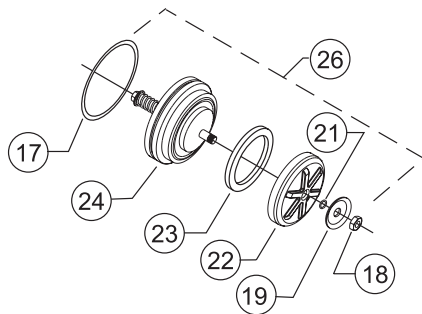
#1 CHECK ASSEMBLY (375 & 475 2 1/2" & 3")
