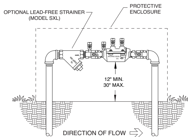
OUTDOOR INSTALLATION
