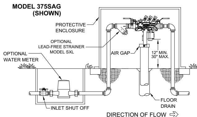
OUTDOOR INSTALLATION
