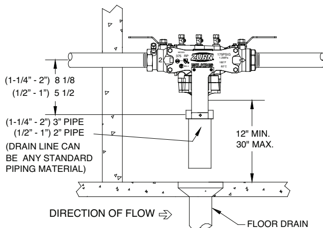
INDOOR INSTALLATION
