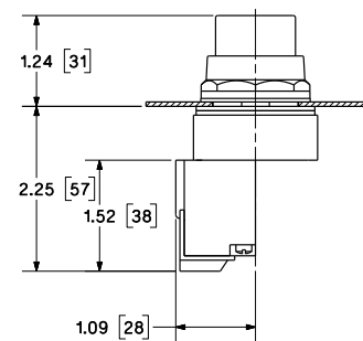
Indicator light plastic lens
