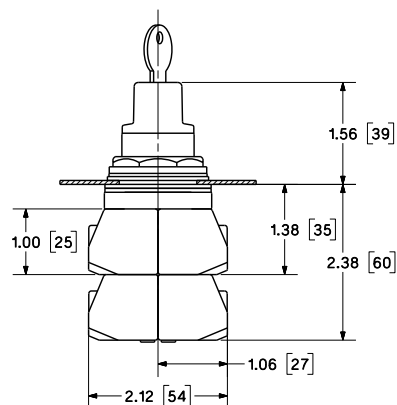
Selector switch keyed
