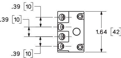
Contact block Dimensions inches, [mm]
