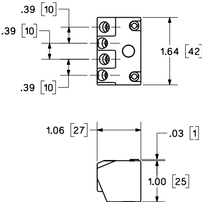
Contact block
