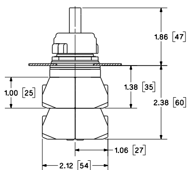
Toggle switch
