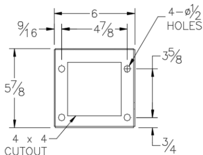
HIDDEN BASEPLATE (Standard)
