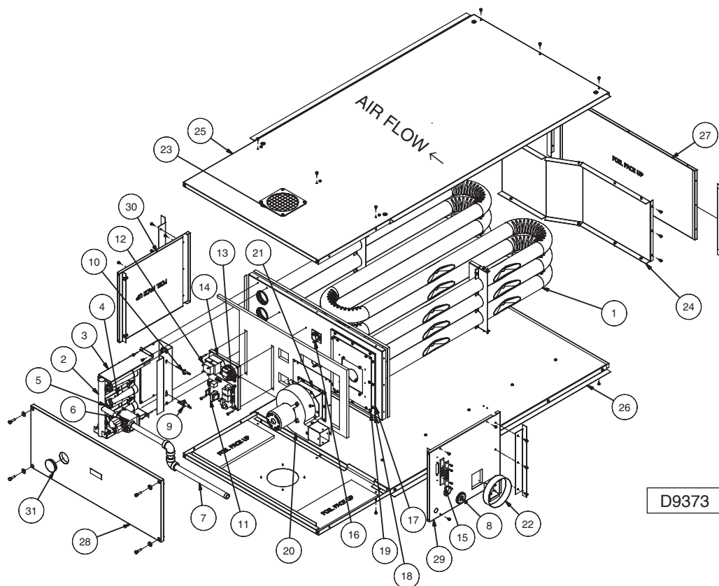
Figure 23 – Exploded View
