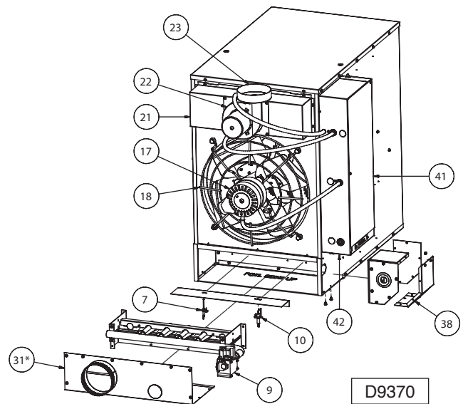
Figure 8 – Rear View
