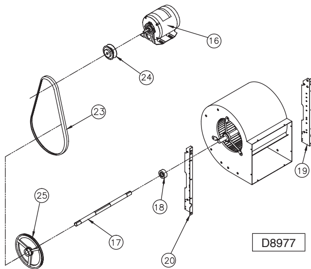
Figure 22 – Blower Assembly
