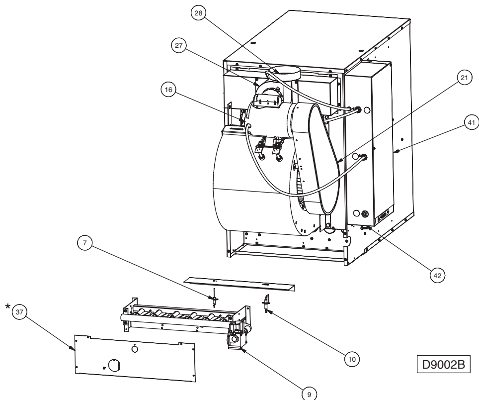
Figure 14 – Rear View
