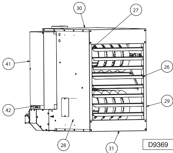
Figure 7 – Front View
