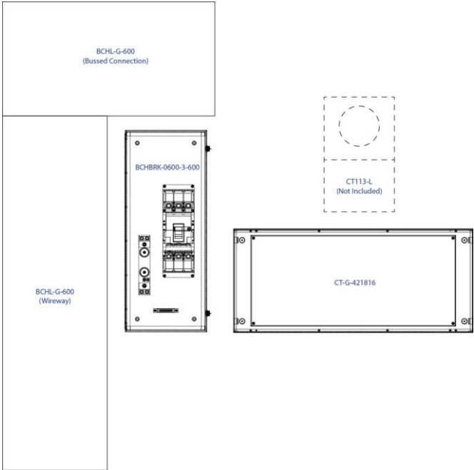
Example of 600A Service Installation
