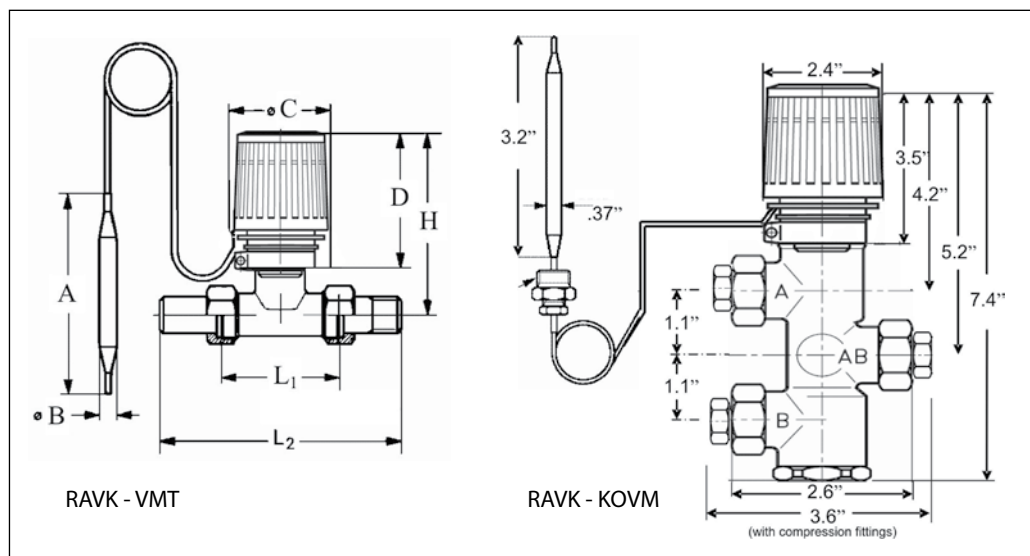
RAVK-VMT Valve
