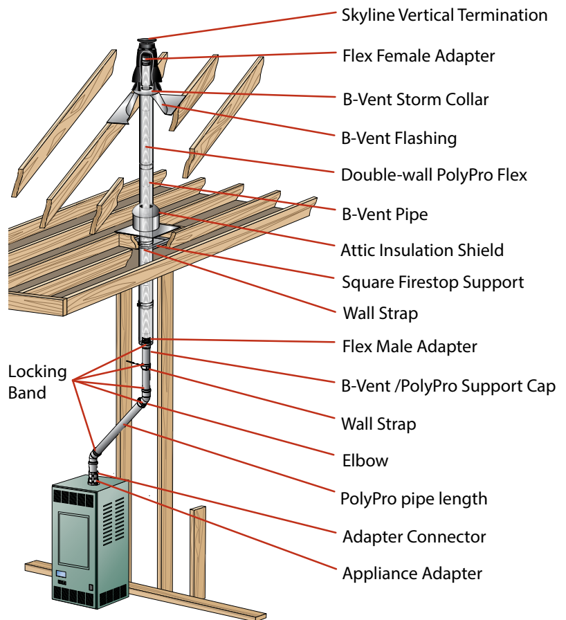
Flex Through B vent as a chase
