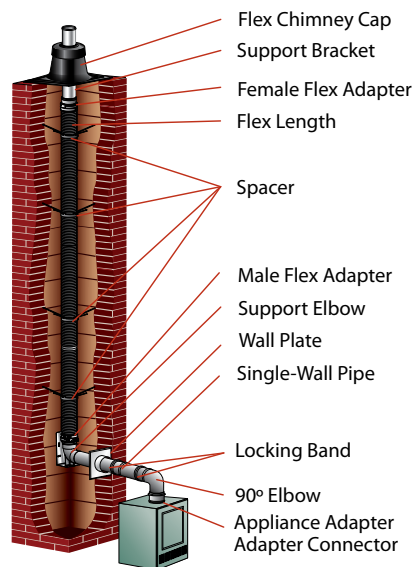
Flex Through Chimney
