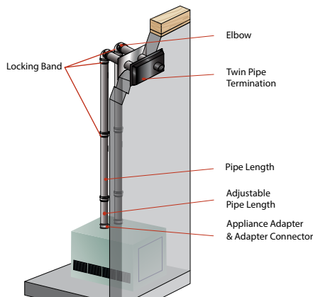
Horizontal Below Grade
