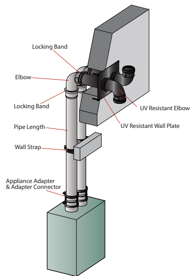
Horizontal Twin Pipe Elbow Termination
