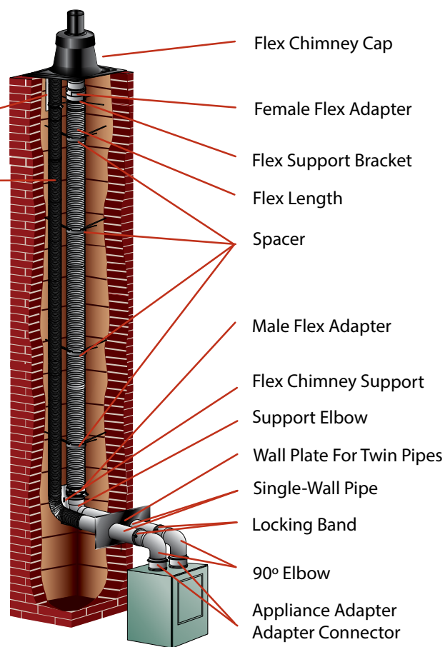
Flex Through Chimney w/Air Intake
