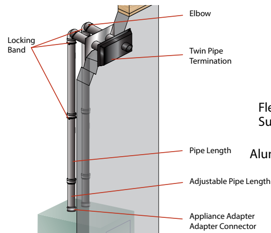
Horizontal Twin Pipe Below Grade
