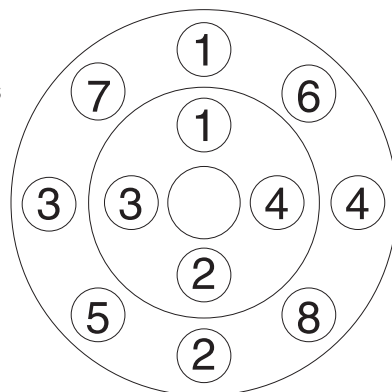
Flange Bolt Tightening Patterns
