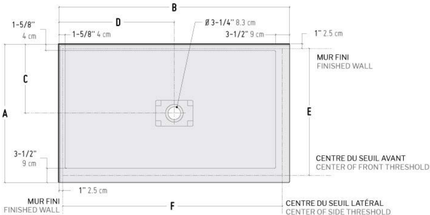
BRIDE DE CARRELAGE TILING FLANGE
