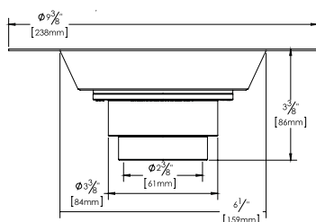
1-1/2" pipe size connection
