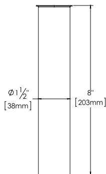
Flanged Tailpiece Attaches to 314DC Series Direct/Offset Bath Wastes.
