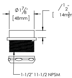
Chrome Plated Brass Nut and Poly Washer to be installed on drain.
