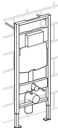
Pre-wall installation, front activation.
