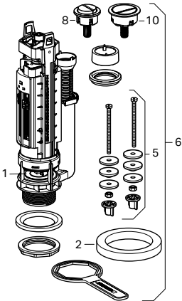
Flushing Valve Type 290 Dual-flush
