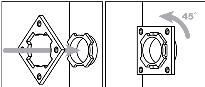
Figure 28 TWIST-LOCK
