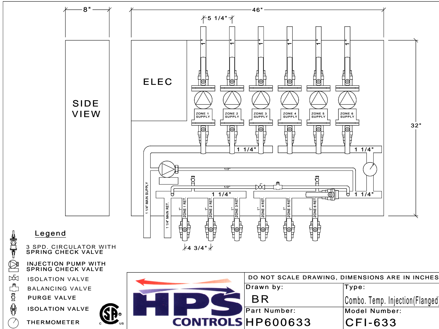
Diagram D [Combo Temp. Injection (Flanged)]
