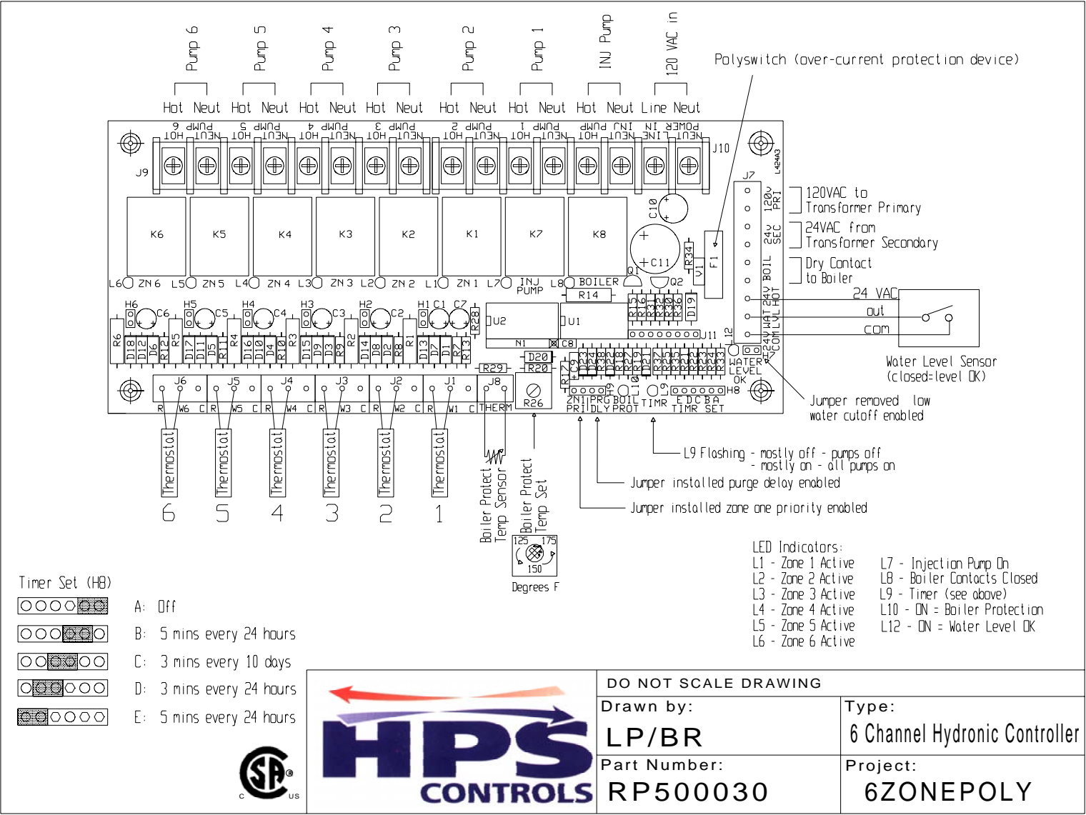
Diagram C (6-Zone Hydronic Controller)
