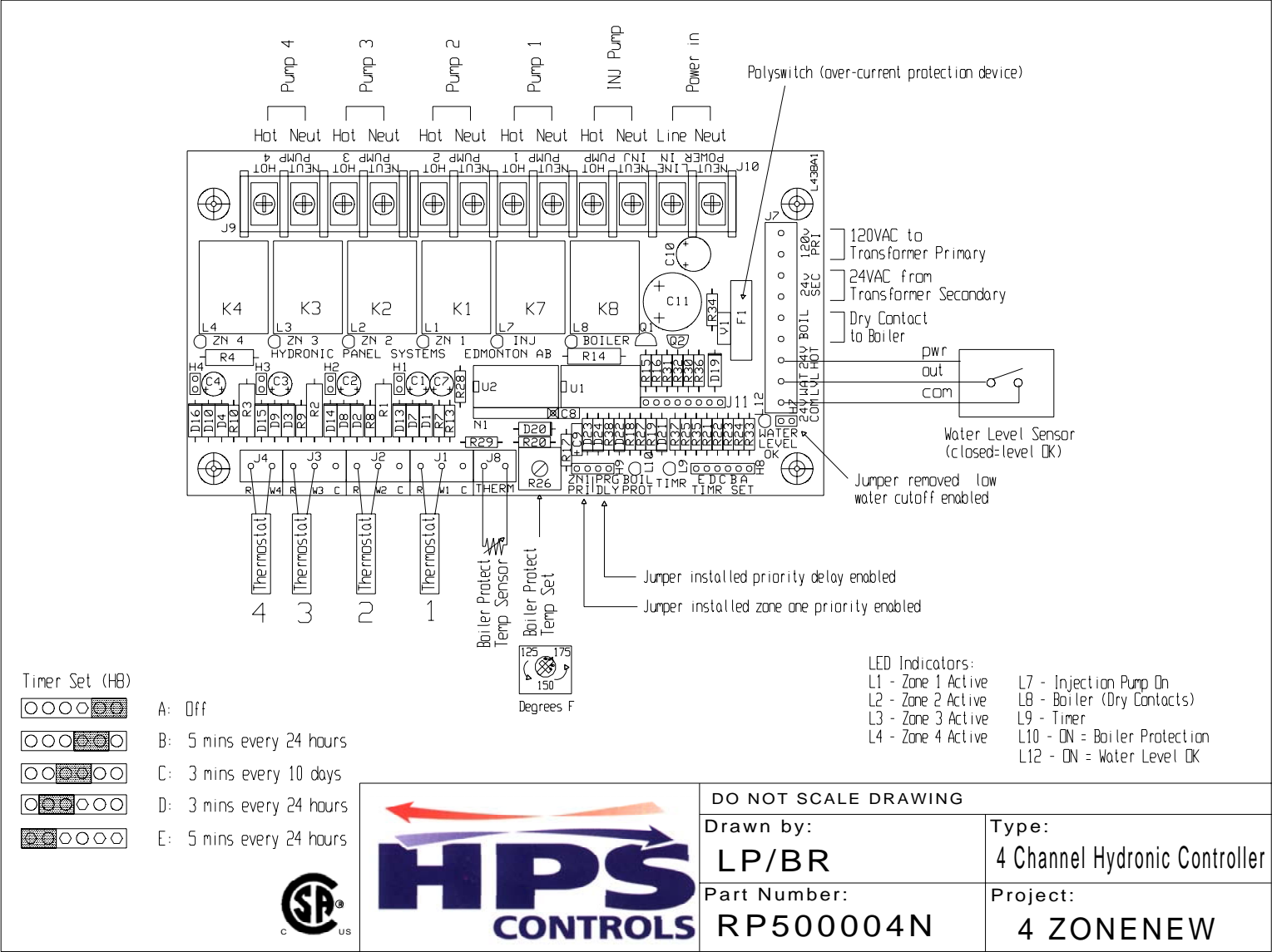
Diagram B (4-Zone Hydronic Controller)
