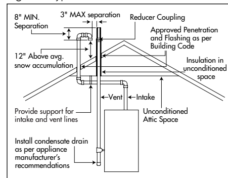
Figure 2 Typical Roof Termination
