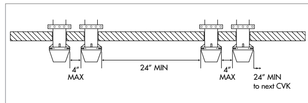
Figure 13: Typical CVK Spacing
