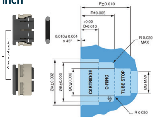
Cavity Dimensional Detail (CTS)
