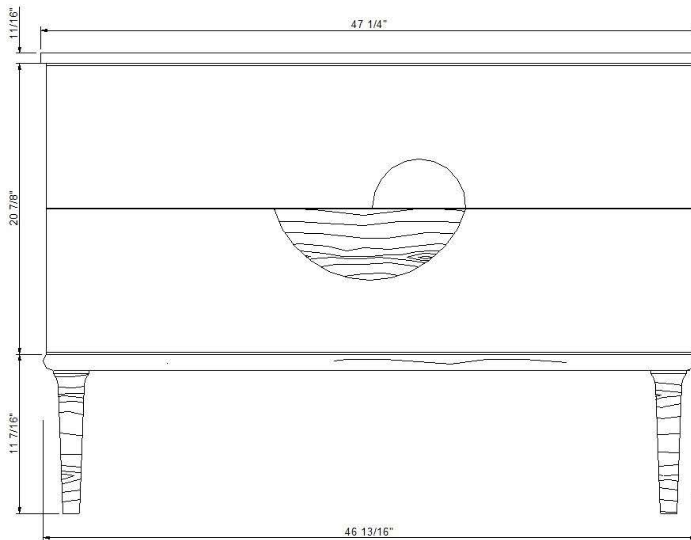
Elevation view
