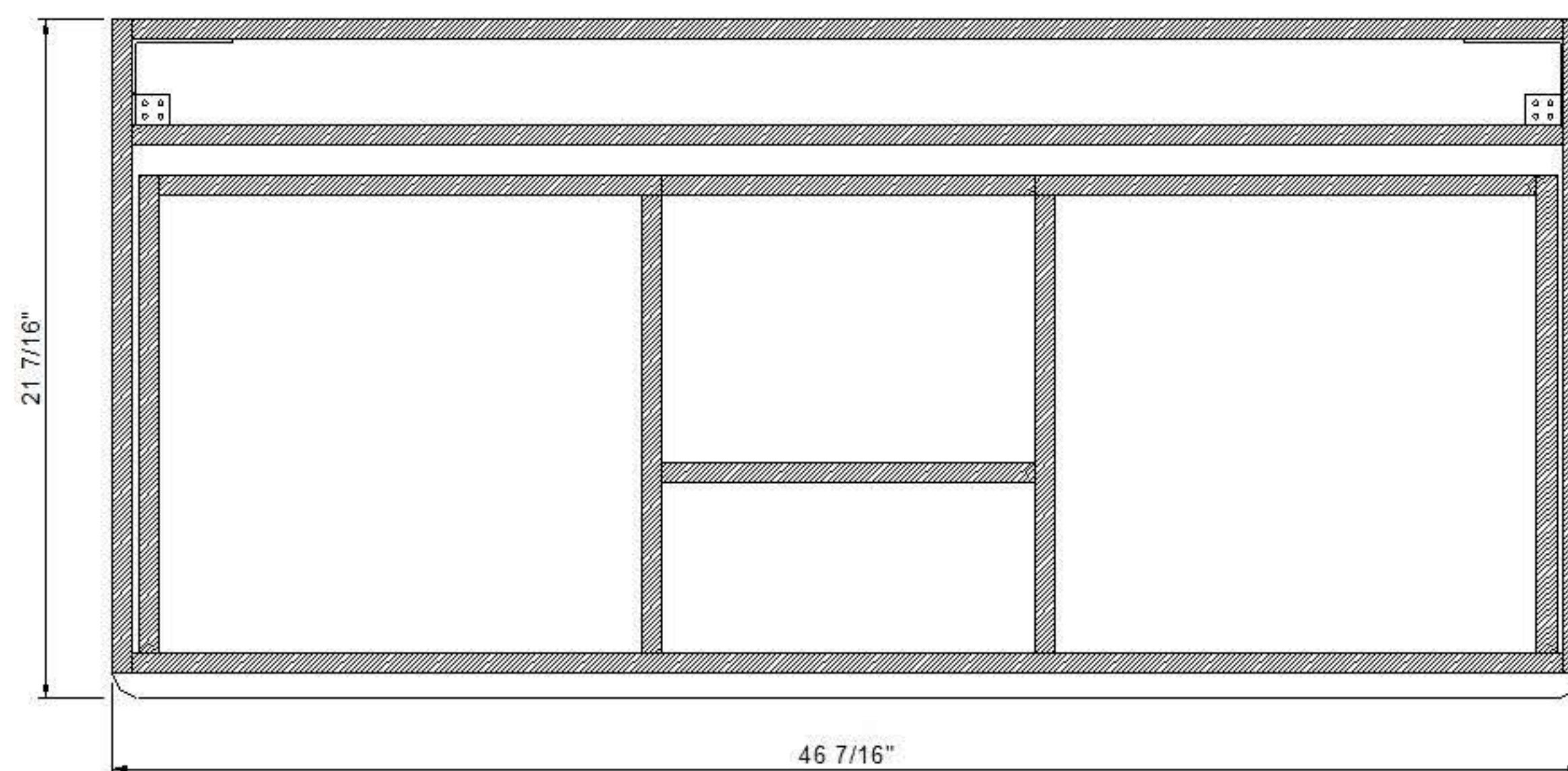
Top view
