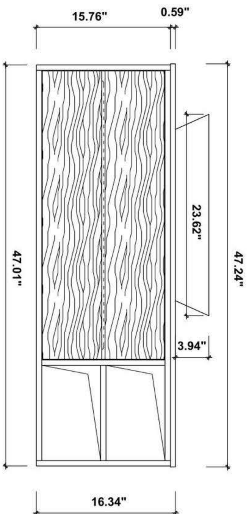
FRONT ELEVATION
