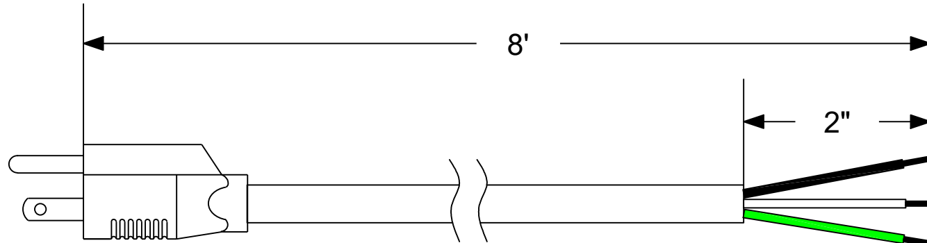
KK1000 NEMA 5-15P STANDARD MOLDED
