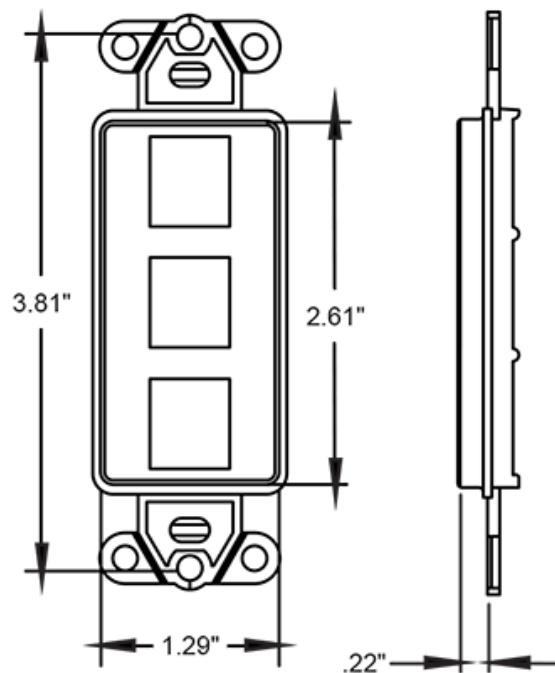
3-Port Insert
