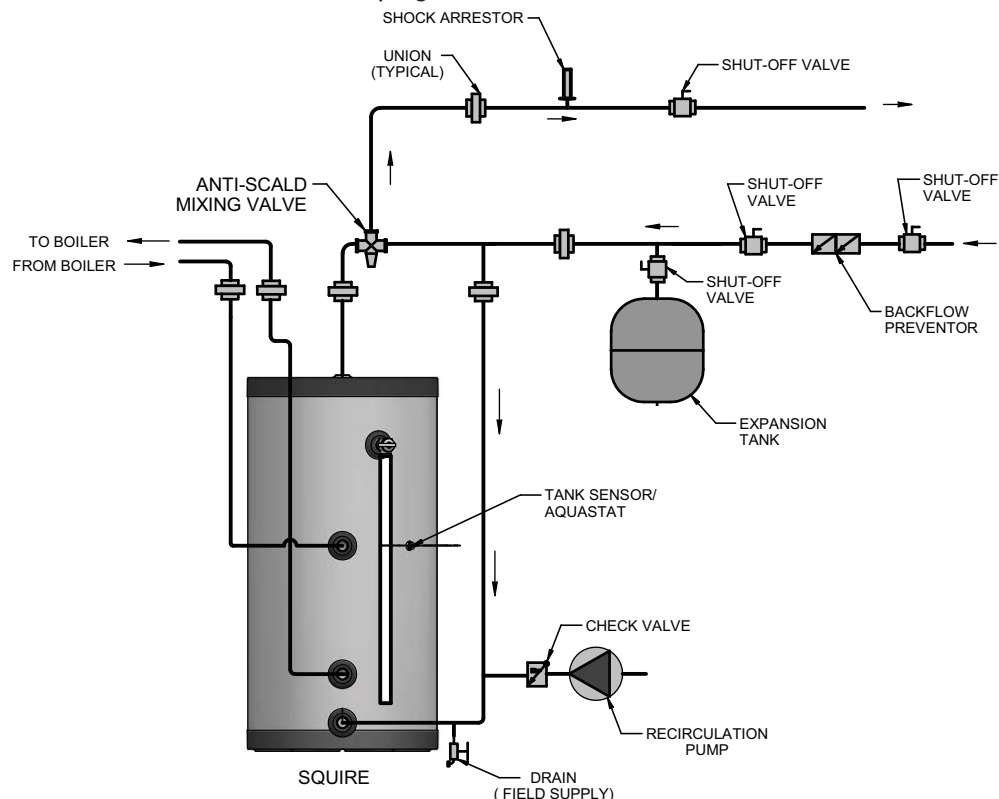
Figure 4-2 Recommended Domestic Water Piping
