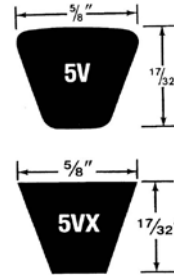
“5V & 5VX” V-Belts
