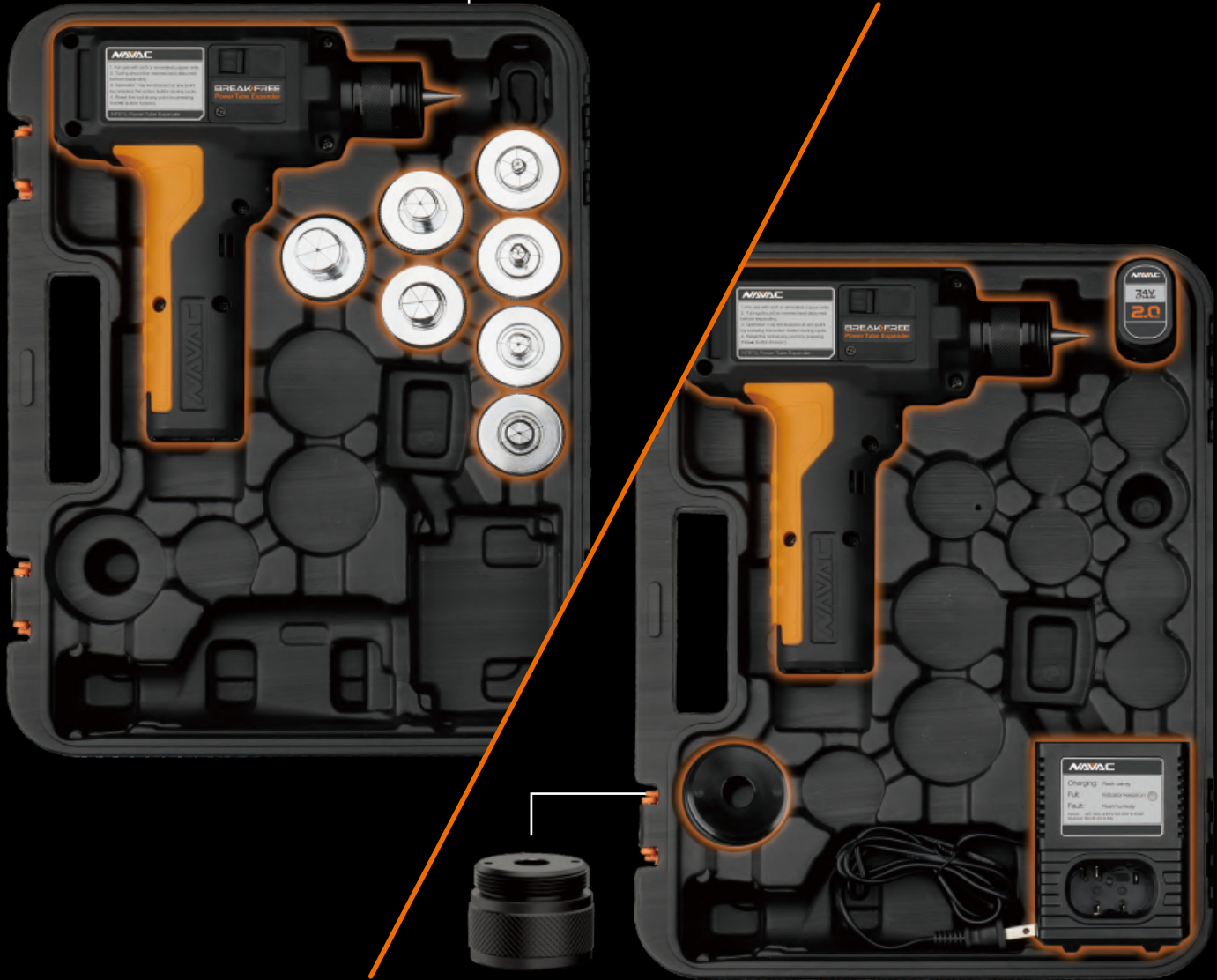
NAQA1 Quick Connect Adapter Expander heads from NTE11H Hydraulic Expander can be shared with NTE11L with a NAQA1 adapter.
