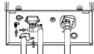
Drain Plugs
