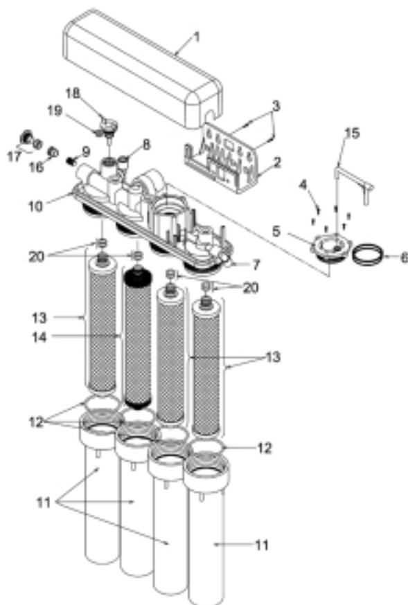
Parts Breakdown, 104 Series Four Vessel Manifold Module
