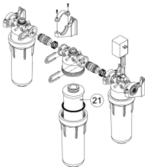
AquaSafe™ Ultraviolet and Mechanical Filtration System 3 Module Unit, 4.5 or 8.5 GPM with Sediment Filter, Carbon Filter and UV Lamp
