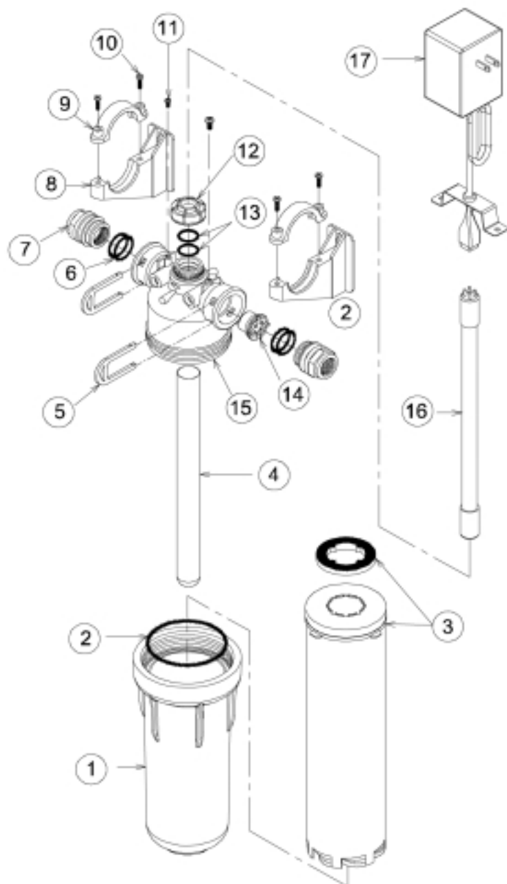
AquaSafe™ Ultraviolet System 1 Module Unit, 4.5 or 8.5 GPM with UV Lamp and Stainless Steel Sleeve
