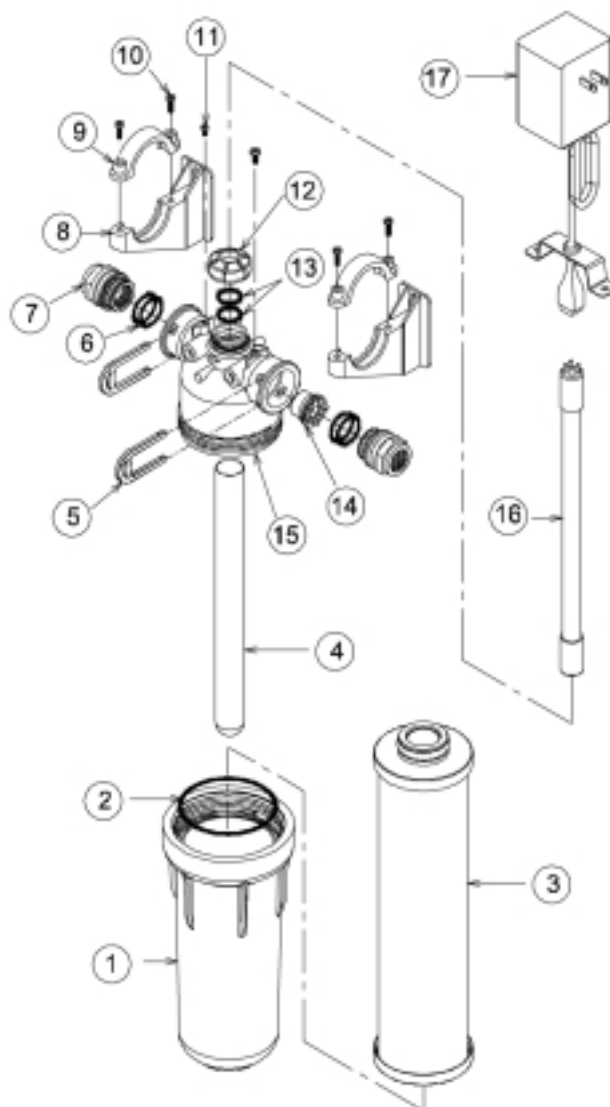
AquaSafe™ Ultraviolet Lamp with Activated Carbon Filter Module Schematic
