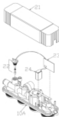
Faucet Smartap® Monitor Module Cover and Flow Switch Assembly
