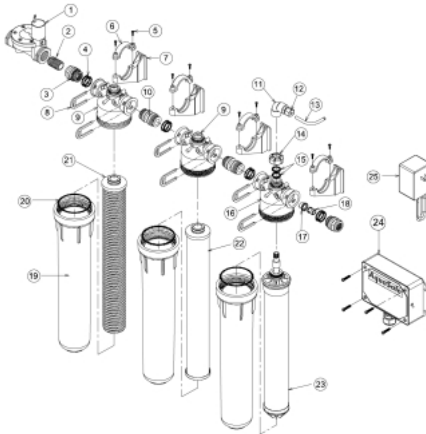
Mechanical Filtration and Reverse Osmosis Modules Installation and Connection Procedures
