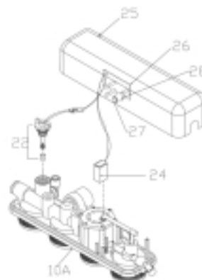
Push Button Smartap® Monitor Module Cover and Flow Switch Assembly
