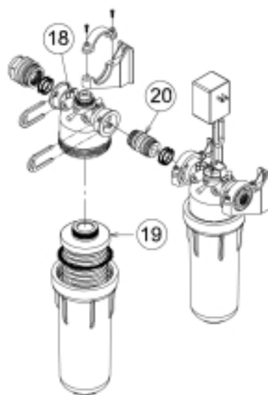
AquaSafe™ Ultraviolet and Mechanical Filtration System 2 Module Unit, 4.5 or 8.5 GPM with Sediment Filter and UV Lamp
