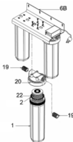
Carbon Filter Components UVBB-3
