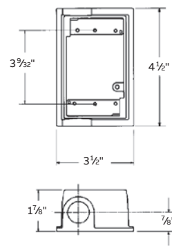
Two-hole flanged box extension adapter
