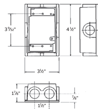
Six-hole flanged box extension adapter
