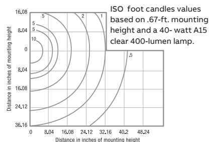
K812BR 10" Height option
