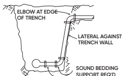
For moderate trench depth
