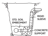
Rigid sleeve for any trench (concrete must support sleeve)
