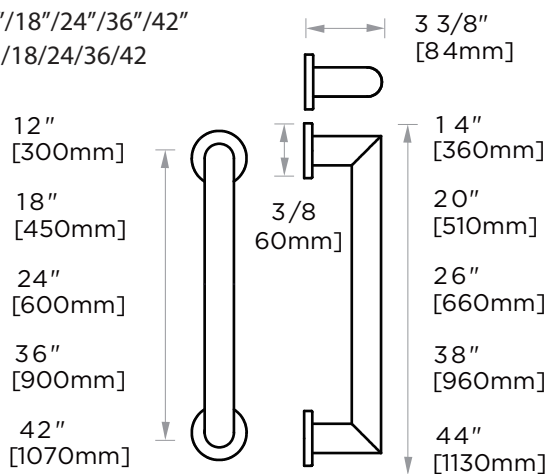
Grab Bar 12"/18"/24"/36"/42" SYD-GB4-12/18/24/36/42
