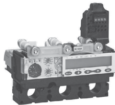
Micrologic Ammeter and Energy Trip Unit
