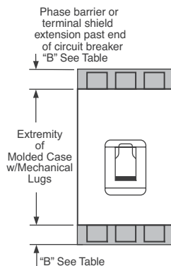
R-Frame Phase Barrier
