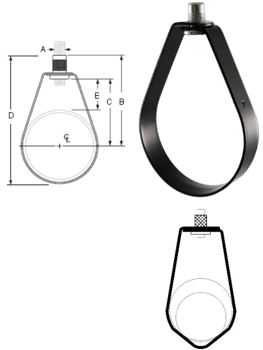
* 1" & 1 1/4" Copper Tube Size Profile
